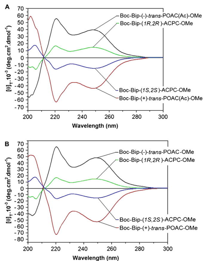
Figure 4. CD spectra (200–300 nm region) of the dipeptides Boc-Bip-( + ) and ( - )- trans -POAC(Ac)-OMe (A), and the corresponding dipeptides with a free nitroxide function Boc-Bip-( + ) and ( - )- trans -POAC-OMe (B), compared to Boc-Bip-(1 R ,2 R )-ACPC-OMe and Boc-Bip-(1 S ,2 S )-ACPC-OMe in MeOH solution (peptide concentration: 1 \times 10^{-3} M).
